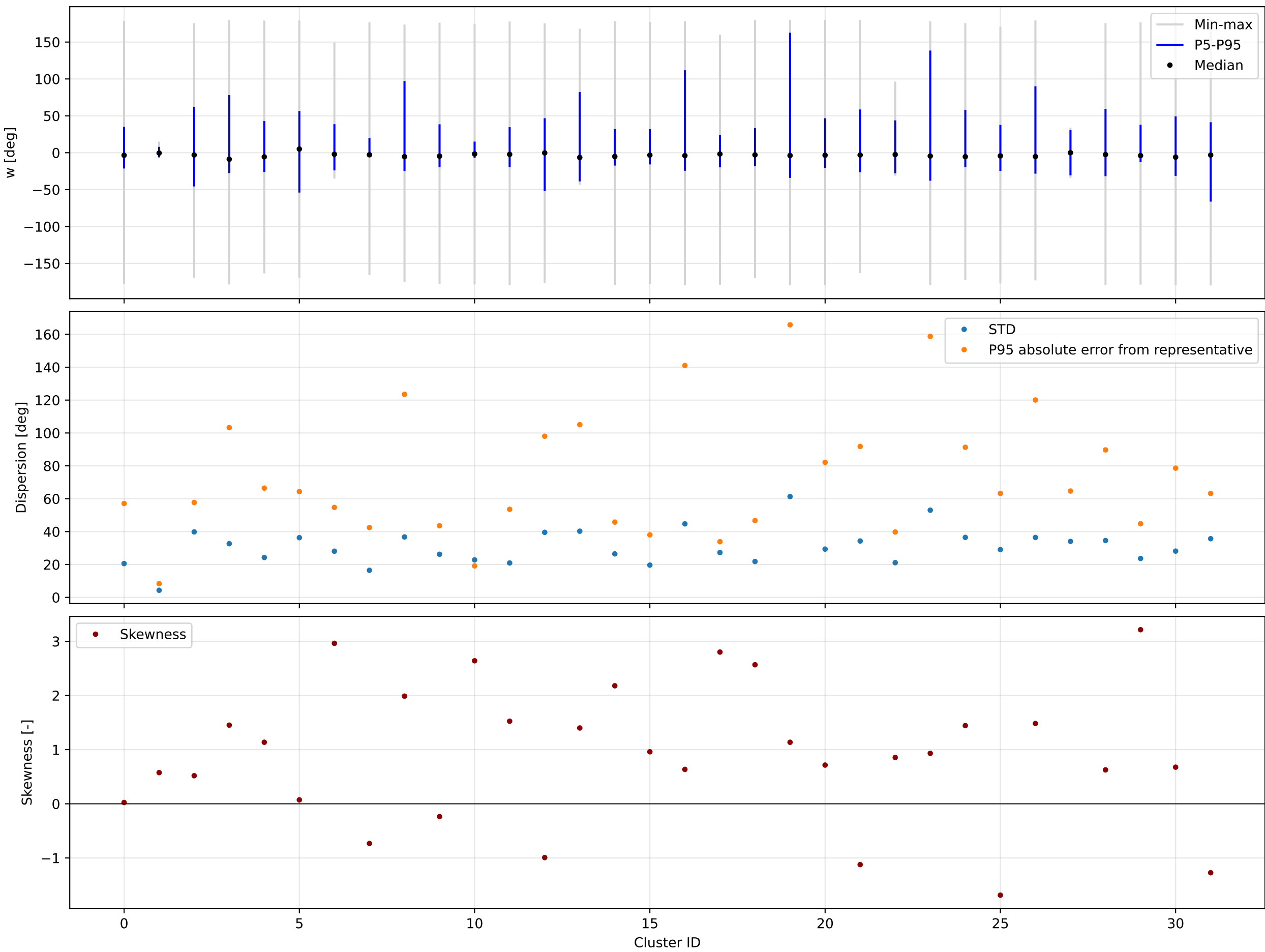
K=32 | forward | w | valid=194050/194058 | offsets from each cluster circular mean
